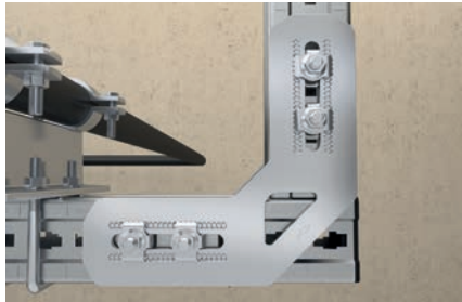
U-rack construction
