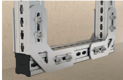
U-rack construction with flat fittings
