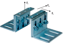
FFPK Saddle max. recom. loads radial F_r = 42000 N lateral F_l = 17500 N
