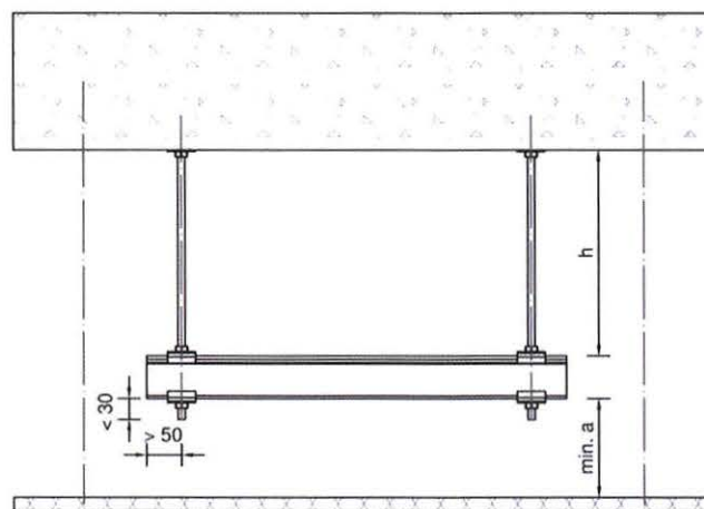
Figure 1 Illustration of use in the intermediate ceiling area – suspended with threaded rods
