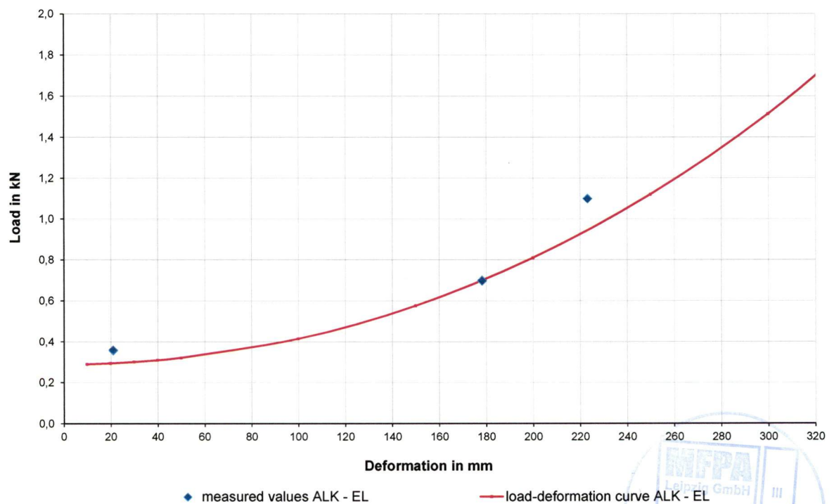
Diagram A2.8 Load-deformation curve for FLS 37/1.2 as cantilever arm ALK 37/1.2 with single load with a fire-resistance period of 30 minutes
