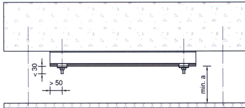
Figure 2 Illustration of use in the intermediate ceiling area – directly fastened to the ceiling
