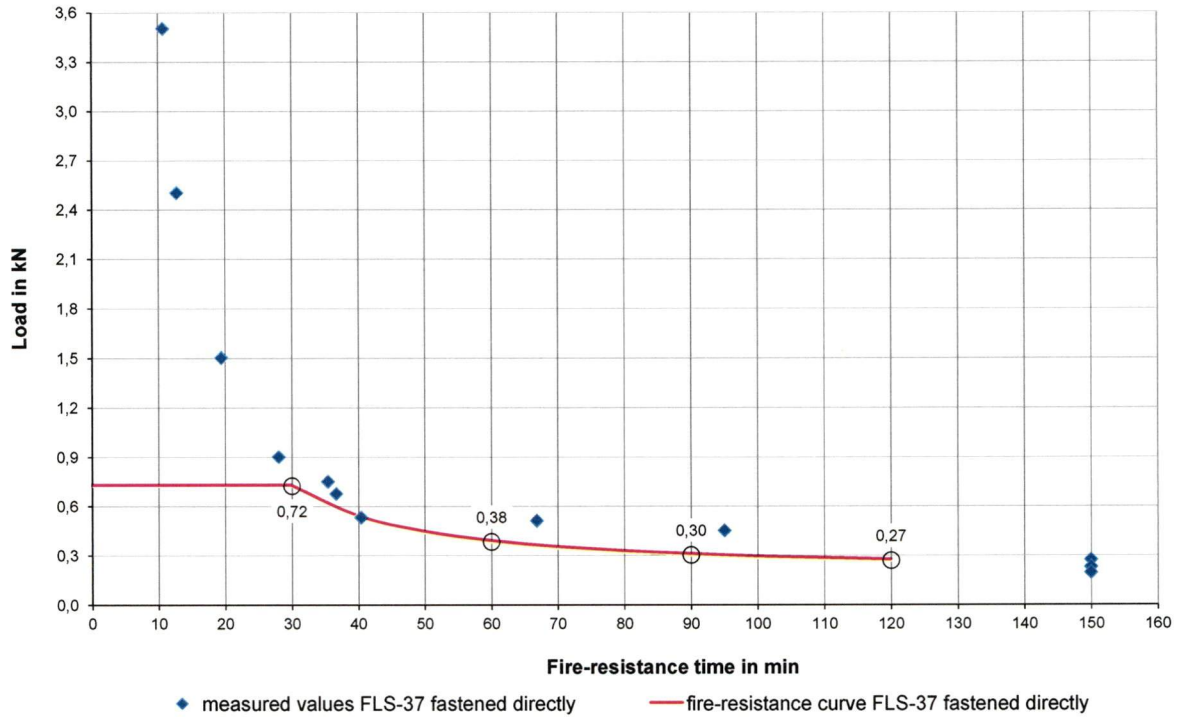
Diagram A2.1 Fire-resistance curve for FLS 37/1.2, fastened directly with triple load
