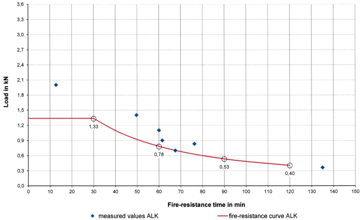
Diagram A2.7 Fire-resistance curve for FLS 37/1.2 as cantilever arm ALK 37/1.2 with single load
