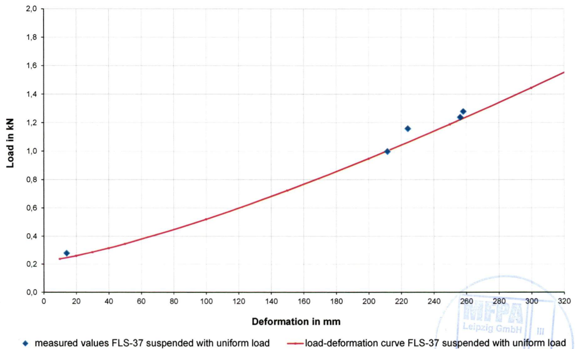
Diagram A2.6 Load-deformation curve for FLS 37/1.2, suspended with uniform load with a fire-resistance period of 30 minutes
