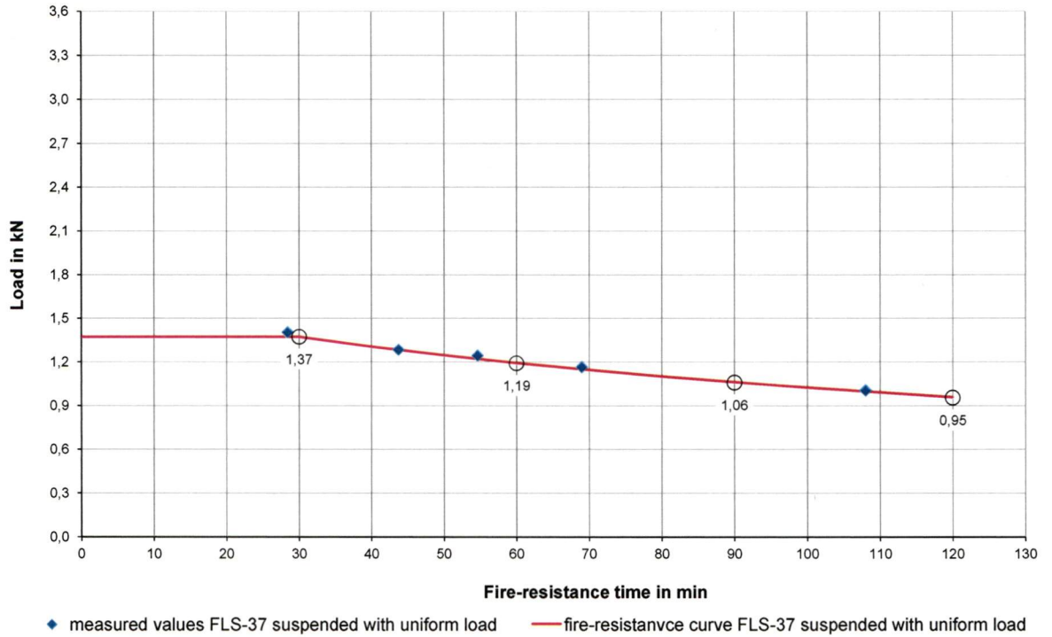
Diagram A2.5 Fire-resistance curve for FLS 37/1.2, suspended with uniform load
