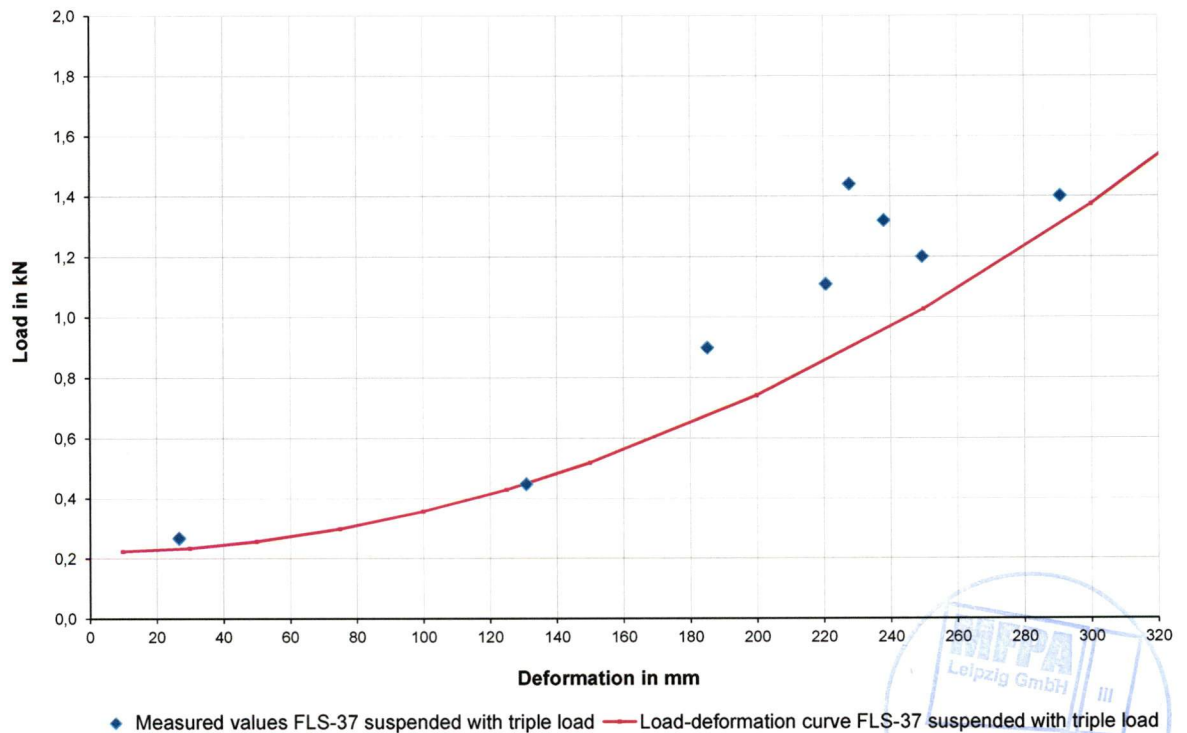
Diagram A2.4 Load-deformation curve for FLS 37/1.2, suspended with triple load with a fire-resistance period of 30 minutes
