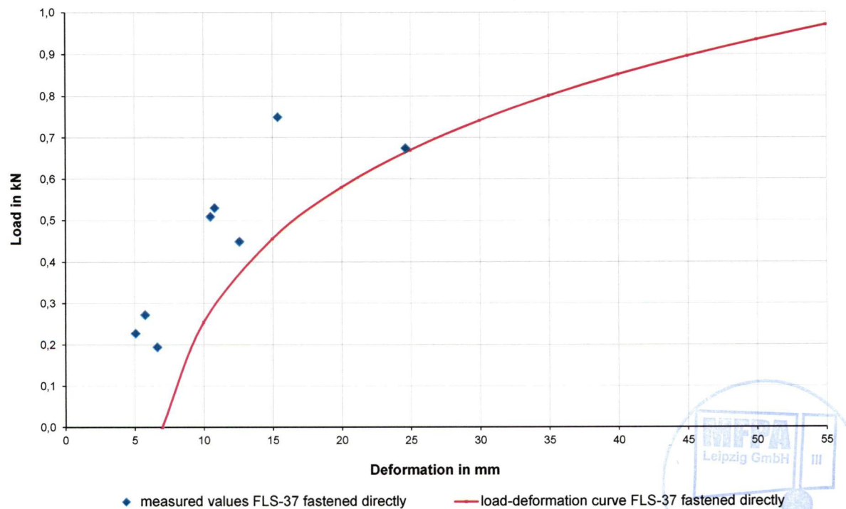
Diagram A2.2 Load-deformation curve for FLS 37/1.2, fastened directly with triple load with a fire-resistance period of 30 minutes
