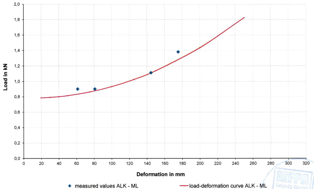
Diagram A2.9 Load-deformation curve for FLS 37/1.2 as cantilever arm ALK 37/1.2 with triple load with a fire-resistance period of 30 minutes
