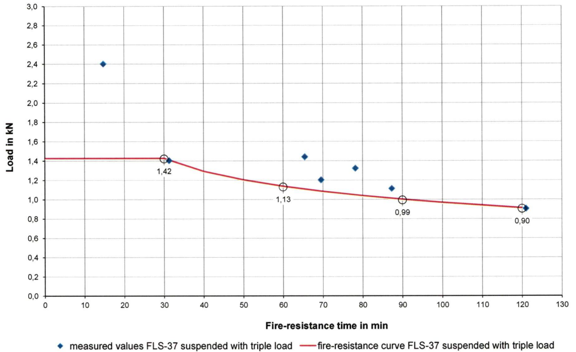
Diagram A2.3 Fire-resistance curve for FLS 37/1.2, suspended with triple load
