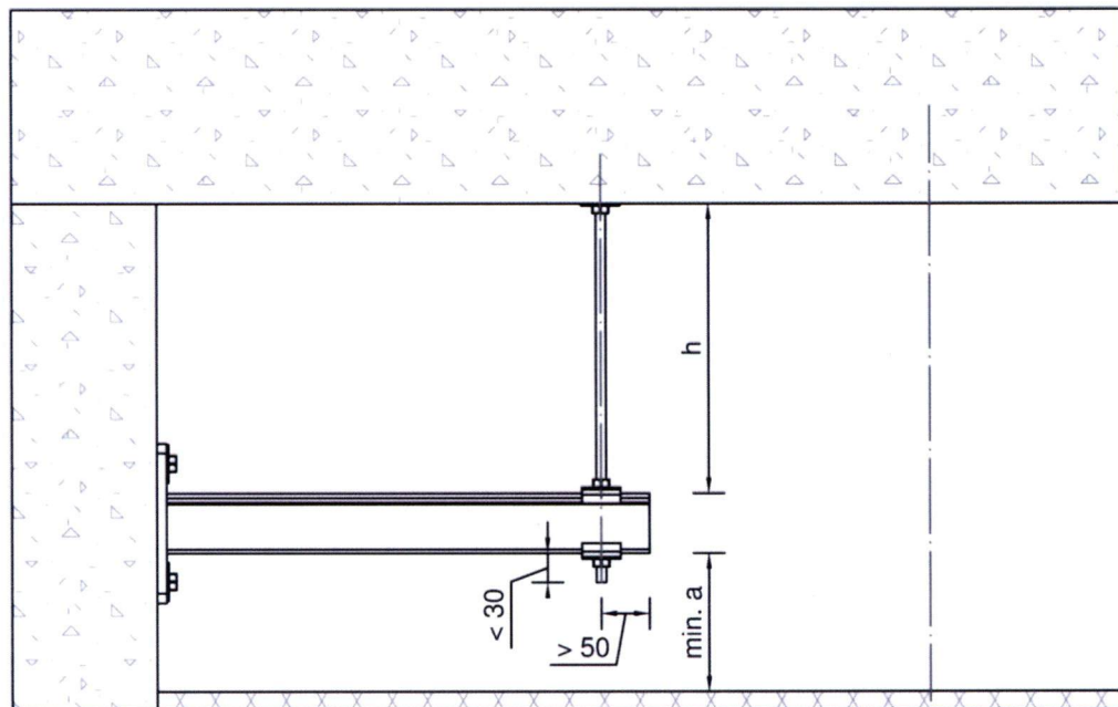
Figure 3 Illustration of use of the fischer cantilever arm ALK 37/1.2 in the intermediate ceiling area
