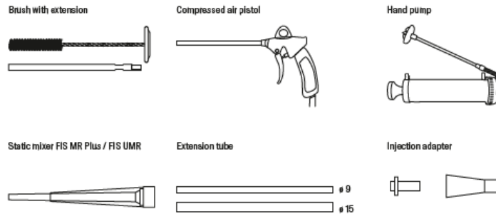
FIGURE 7—FIS SB INSTALLATION INFORMATION (Continued)
