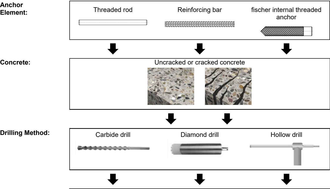
FIGURE 4—INSTALLATION PARAMETERS (CONTINUED)
