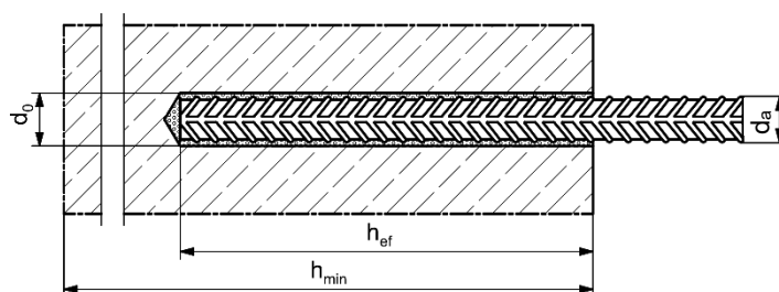
FIGURE 4—INSTALLATION PARAMETERS
