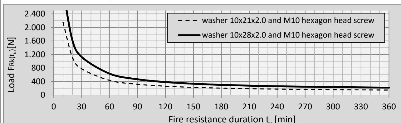
Figure D 1.1: Functional curves of the pull-through resistance FR_k(t_u) through the slotted holes in the channel back under fire exposure
