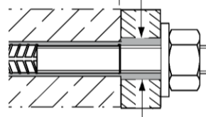
UPAT rebar anchor Push through anchor (annular gap filled with mortar)
