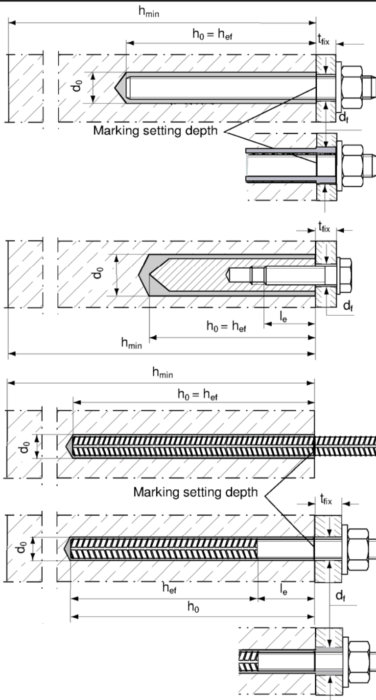
fischer threaded rod FIS A or RGM Pre-positioned anchorage
