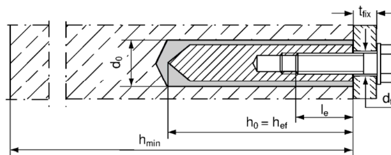
fischer internal threaded anchor RG MI Only pre-positioned anchorage
