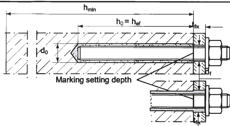
fisher threaded rod FIS A or RGM Pre-positioned anchorage
