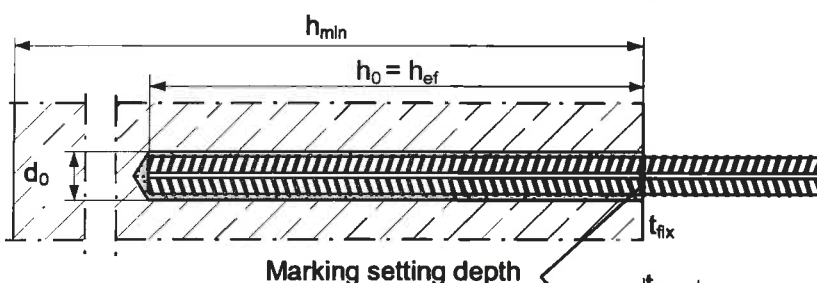
Reinforcing bar
