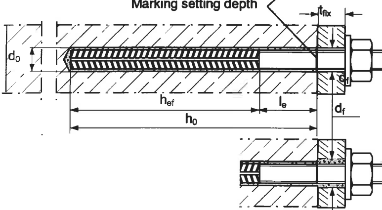
fisher rebar anchor FRA Pre-positioned anchorage
