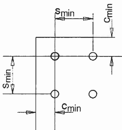
Scheme of distances and spacing
