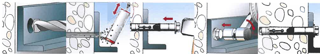
Installation instruction FH II 10 - 32 S and FH II 10-24 S A4
