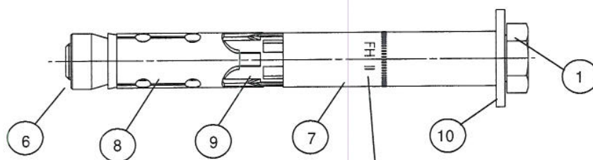
Screw type S FH II 12 - 24
