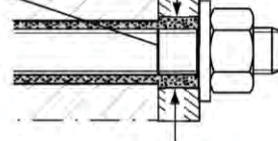
Anchor rod Push through anchor (annular gap filled with mortar) Only injection mortar system FIS SB
