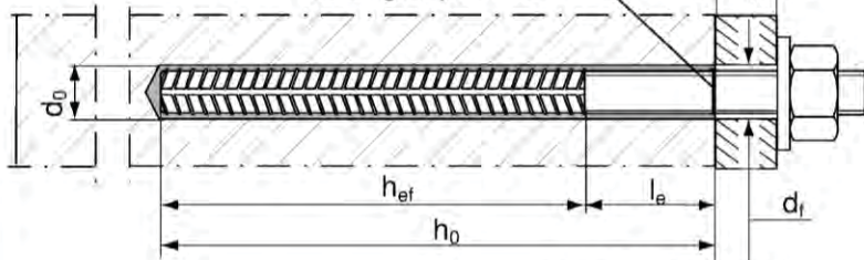
fischer rebar anchor FRA Pre-positioned anchor Only injection mortar system FIS SB
