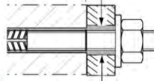
fischer rebar anchor FRA Push through anchor (annular gap filled with mortar) Only injection mortar system FIS SB
