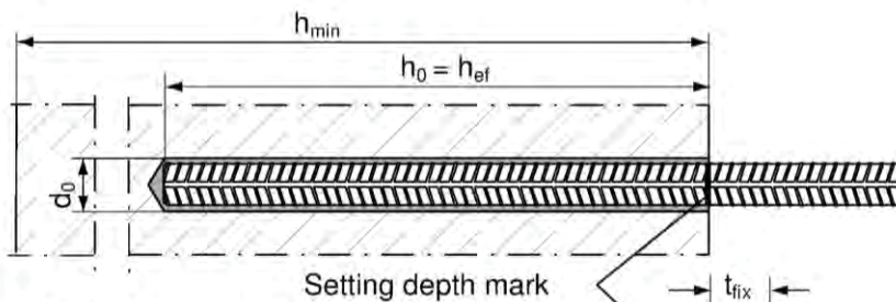
Reinforcing bar Only injection mortar system FIS SB
