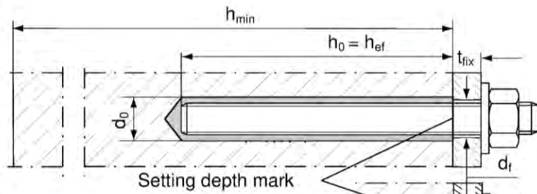
Anchor rod Pre-positioned anchor
