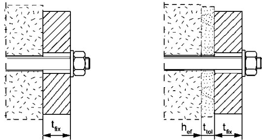
Installation with render bridge
