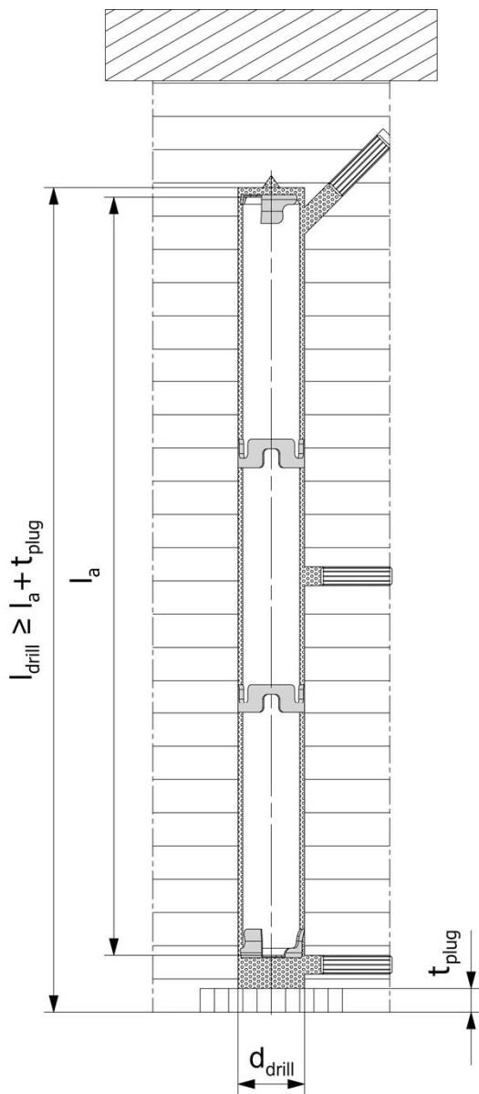
Fischer Anchor rod FIS A and commercial standard threaded rod
