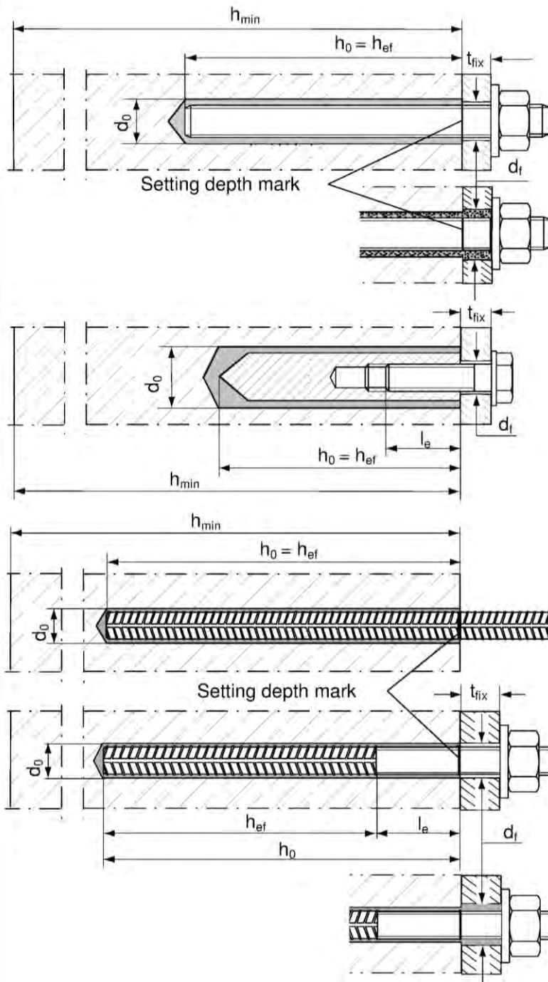
Anchor rod Pre-positioned anchor
