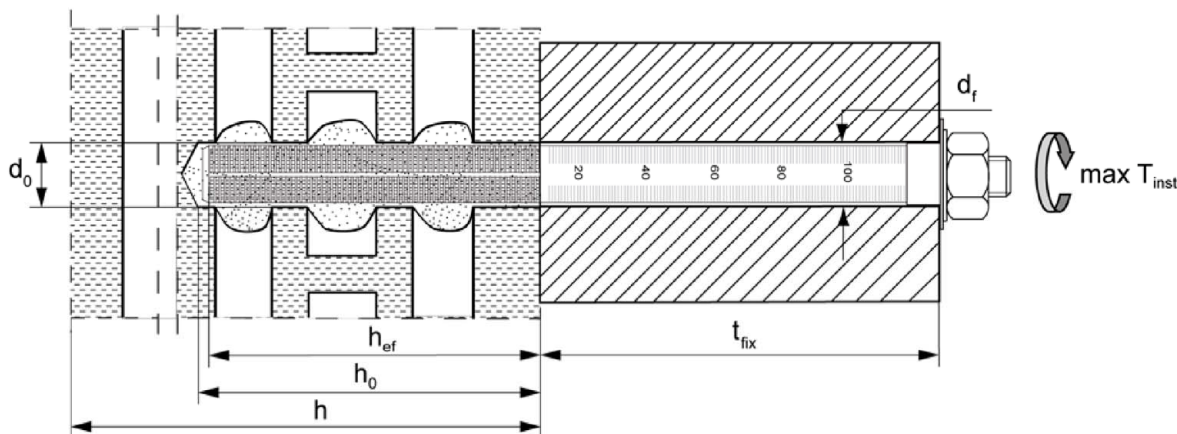
Anchor rod with perforated sleeve
