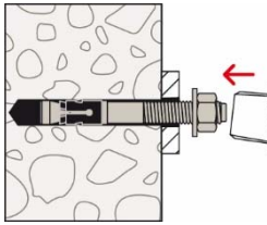
5.a: Set the fastener e.g. with hammer
