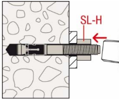
5.1: Set the fastener through the setting gauge and fixture
