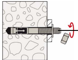
5.3: Remove nut
