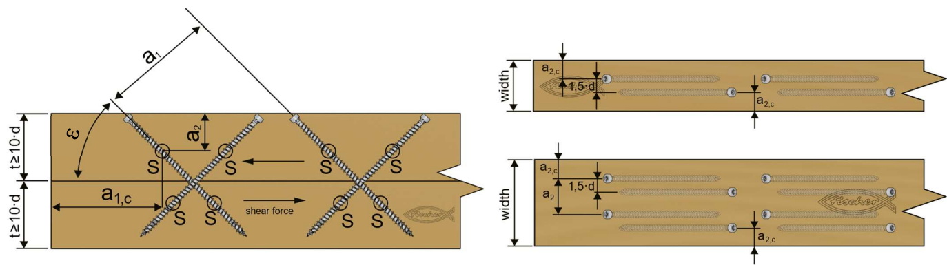
Figure E2.1: Mechanically jointed beam with crossing screws (figures not to scale)
