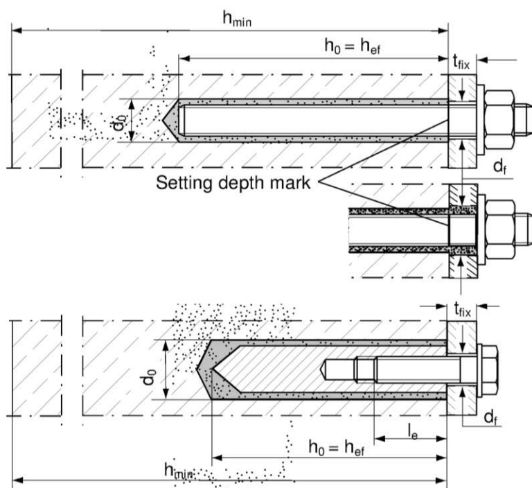
Anchor rod Pre-positioned anchor
