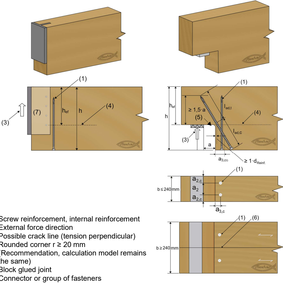
Figure H1.1: Notched beams, reinforcements with internal screws (figures not to scale)
