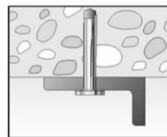
4: Installed fastener
