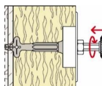
4. Set anchor by setting tool with the machine
