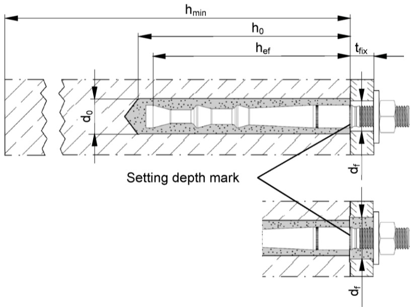
Highbond-Anchor FHB II Inj-A L Pre-positioned anchor
