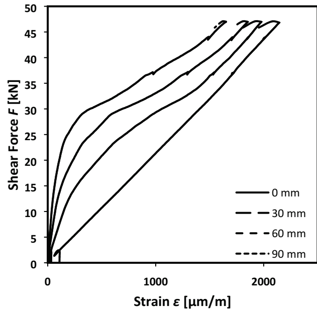
Figure C26.2: Shear-force-Strain curves of shear resistance measurements of the anchorage of FRS-L-S CFRP strips externally bonded to concrete of class C12/15 along the bond length. Strain measurement at 0, 30, 60, 90 mm distances from the load application point.
