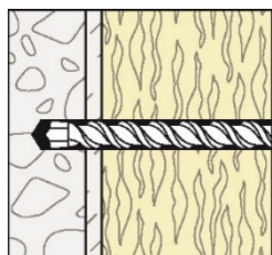
1. Drill hole by corresponding drilling method
