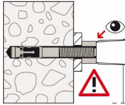
5.2: Check offset
