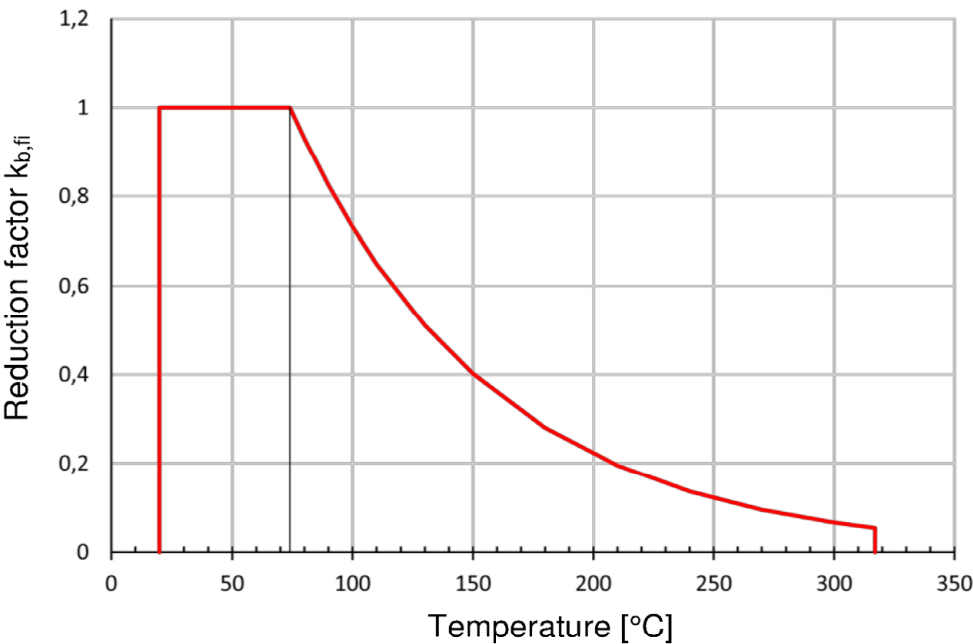
Figure C3.1: Example graph of reduction factor k_{b,fi}(\theta) for concrete class C20/25 for good bond conditions
