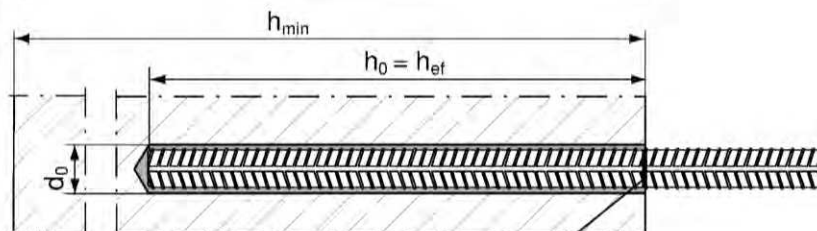
Reinforcing bar
