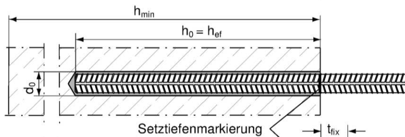
Reinforcing bar
