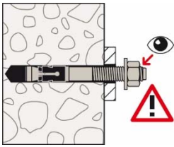
5.1: Check setting position: Visible one turn of a thread
