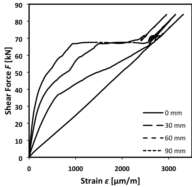
Figure C29.1: Shear-force-strain curves of shear resistance measurements of the anchorage of FRS-L-H CFRP strips externally bonded to concrete of class C30/37 along the bond length. Strain measurement at 0, 30, 60, 90 mm distances from the load application point.
