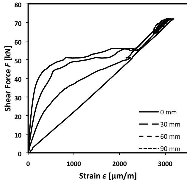
Figure C28.2: Shear-force-strain of shear resistance measurements of the anchorage of FRS-L-S CFRP strips externally bonded to concrete of class C30/37 along the bond length. Strain measurement at 0, 30, 60, 90 mm distances from the load application point.
