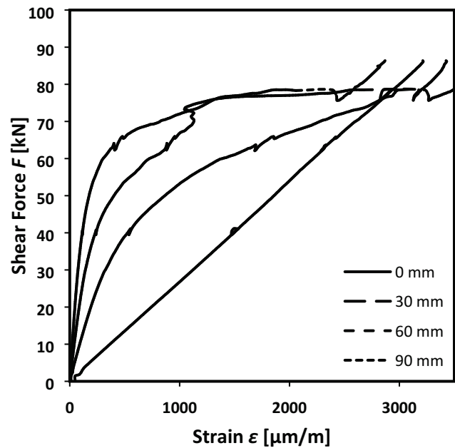
Figure C31.1: Shear-force-strain curves of shear resistance measurements of the anchorage of FRS-L-H CFRP strips externally bonded to concrete of class C50/60 along the bond length. Strain measurement at 0, 30, 60, 90 mm distances from the load application point.
