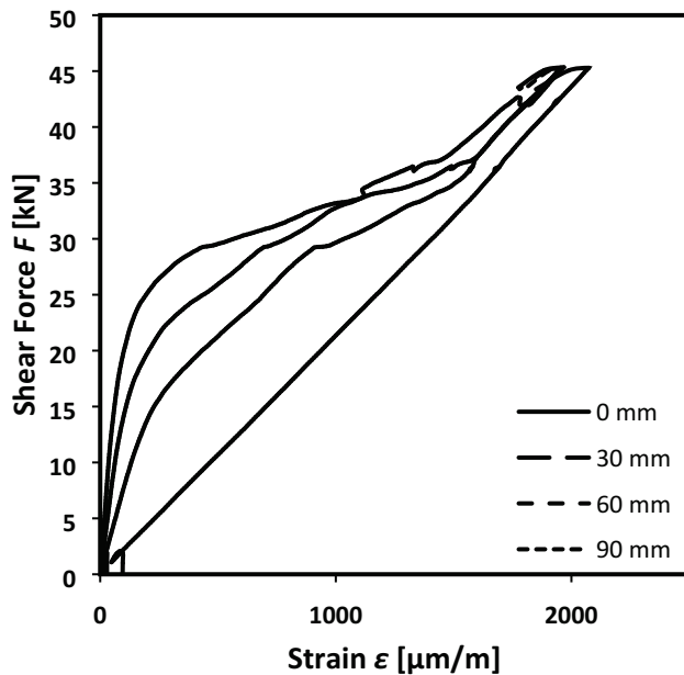
Figure C26.2: Shear-force-Strain curves of shear resistance measurements of the anchorage of FRS-L-S CFRP strips externally bonded to concrete of class C12/15 along the bond length. Strain measurement at 0, 30, 60, 90 mm distances from the load application point.
