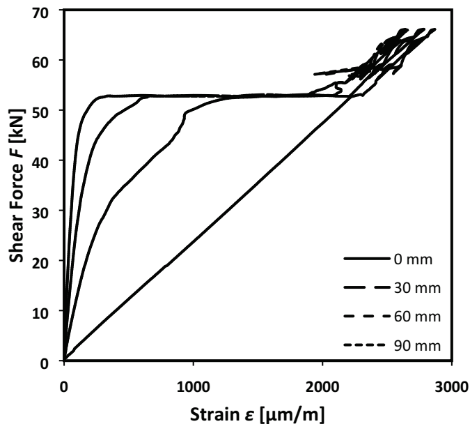
Figure C30.2: Shear-force-strain curves of shear resistance measurements of the anchorage of FRS-L-S CFRP strips externally bonded to concrete of class C50/60 along the bond length. Strain measurement at 0, 30, 60, 90 mm distances from the load application point.
