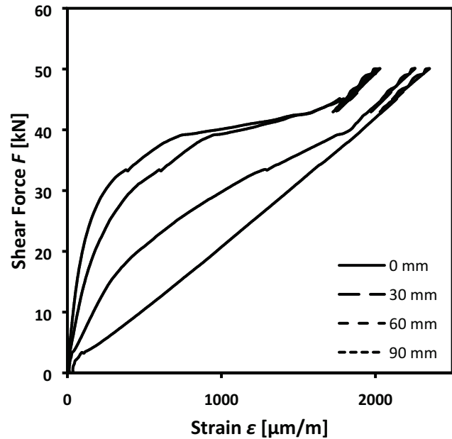
Figure C26.1: Shear-force-strain curves of shear resistance measurements of the anchorage of FRS-L-S CFRP strips externally bonded to concrete of class C12/15 along the bond length. Strain measurement at 0, 30, 60, 90 mm distances from the load application point.
