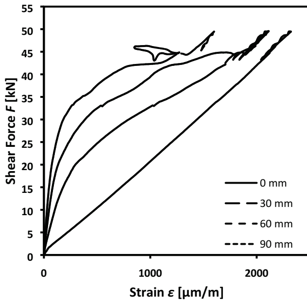
Figure C26.1: Shear-force-strain curves of shear resistance measurements of the anchorage of FRS-L-S CFRP strips externally bonded to concrete of class C12/15 along the bond length. Strain measurement at 0, 30, 60, 90 mm distances from the load application point.
