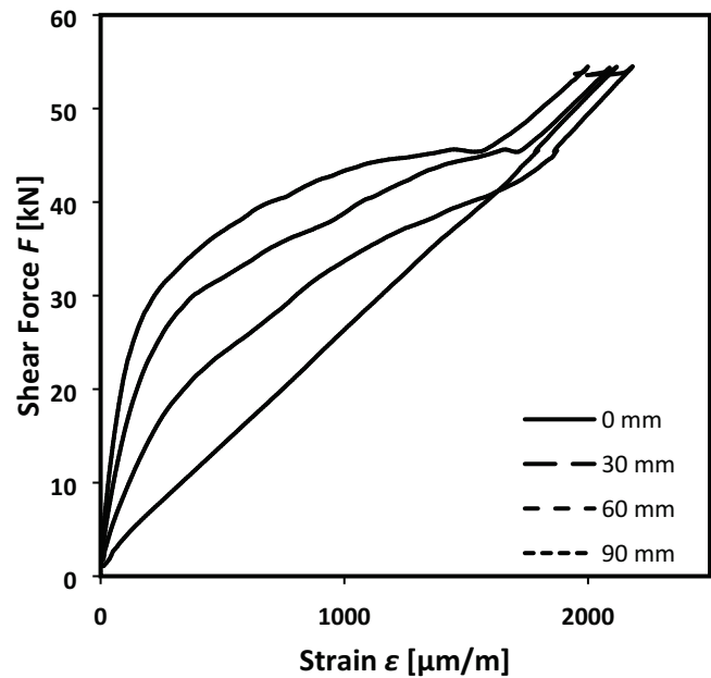
Figure C27.1: Shear-force-strain curves of shear resistance measurements of the anchorage of FRS-L-H CFRP strips externally bonded to concrete of class C12/15 along the bond length. Strain measurement at 0, 30, 60, 90 mm distances from the load application point.
