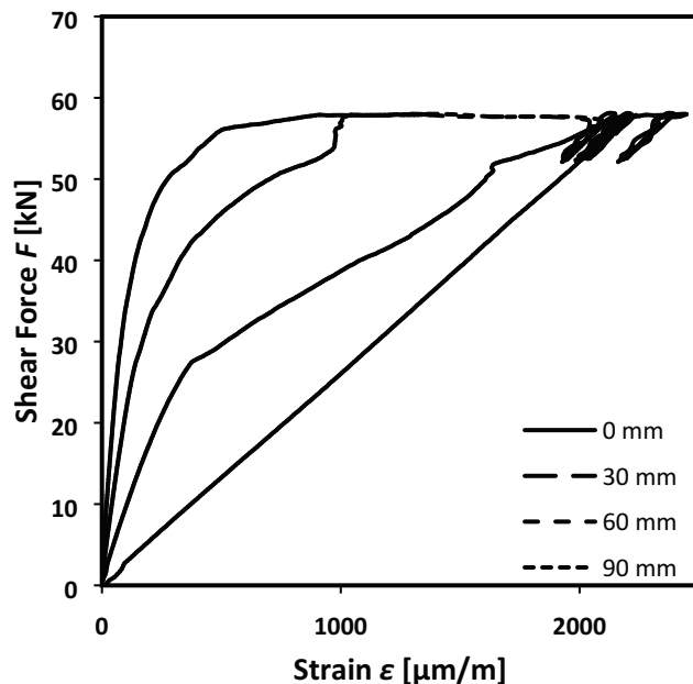
Figure C31.2: Shear-force-strain curves of shear resistance measurements of the anchorage of FRS-L-H CFRP strips externally bonded to concrete of class C50/60 along the bond length. Strain measurement at 0, 30, 60, 90 mm distances from the load application point.
