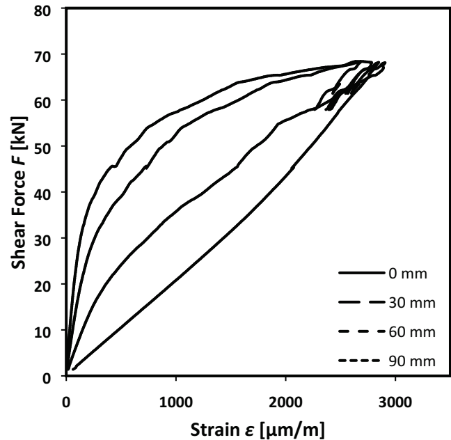
Figure C28.1: Shear-force-strain curves of shear resistance measurements of the anchorage of FRS-L-S CFRP strips externally bonded to concrete of class C30/37 along the bond length. Strain measurement at 0, 30, 60, 90 mm distances from the load application point.
