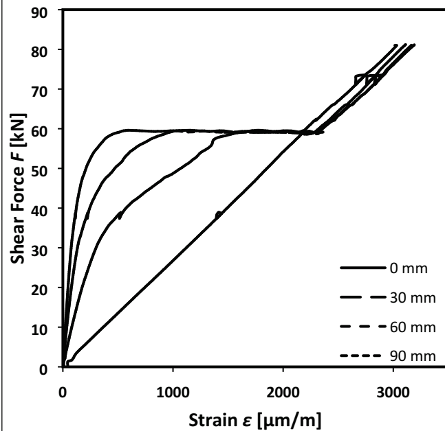
Figure C31.1: Shear-force-strain curves of shear resistance measurements of the anchorage of FRS-L-H CFRP strips externally bonded to concrete of class C50/60 along the bond length. Strain measurement at 0, 30, 60, 90 mm distances from the load application point.
