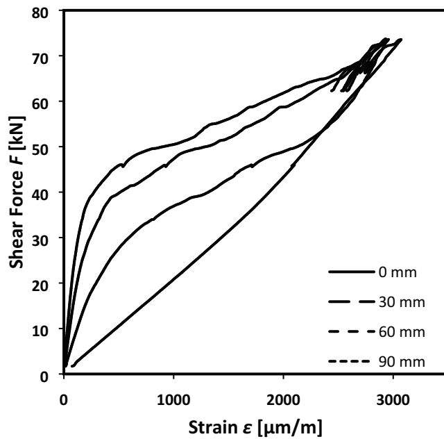
Figure C28.1: Shear-force-strain curves of shear resistance measurements of the anchorage of FRS-L-S CFRP strips externally bonded to concrete of class C30/37 along the bond length. Strain measurement at 0, 30, 60, 90 mm distances from the load application point.
