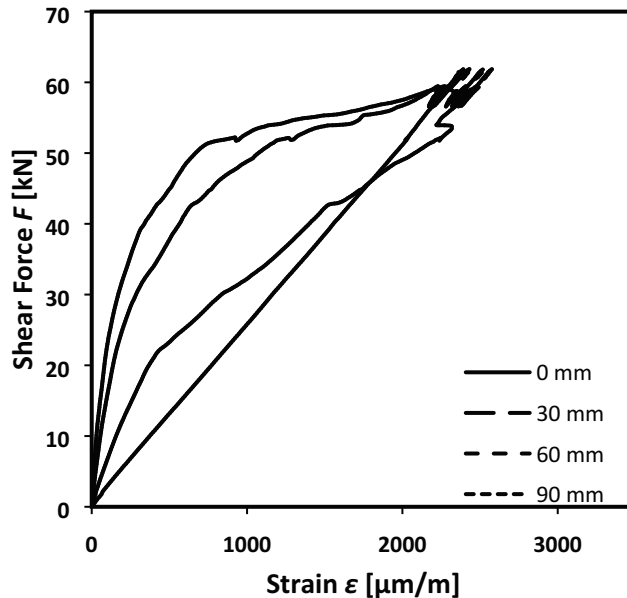
Figure C29.2: Shear-force-strain curves of shear resistance measurements of the anchorage of FRS-L-H CFRP strips externally bonded to concrete of class C30/37 along the bond length. Strain measurement at 0, 30, 60, 90 mm distances from the load application point.
