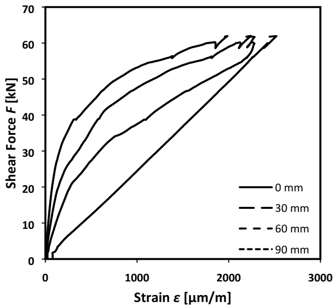
Figure C27.2: Shear-force-strain curves of shear resistance measurements of the anchorage of FRS-L-H CFRP strips externally bonded to concrete of class C12/15 along the bond length. Strain measurement at 0, 30, 60, 90 mm distances from the load application point.
