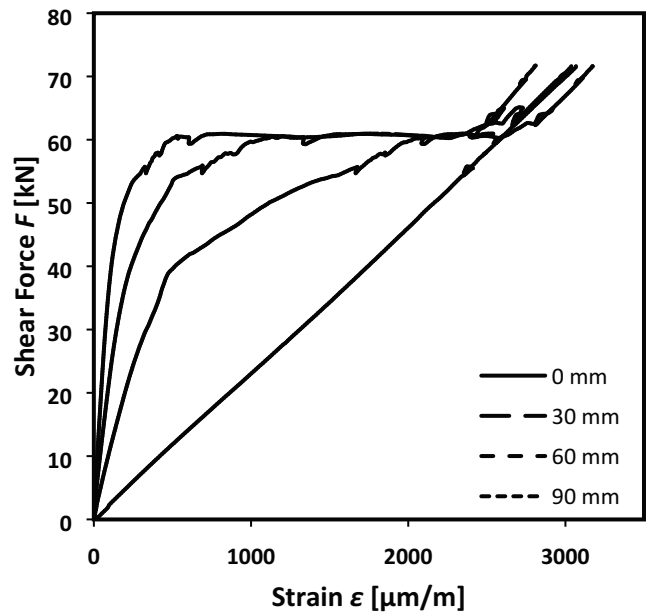
Figure C30.1: Shear-force-strain curves of shear resistance measurements of the anchorage of FRS-L-S CFRP strips externally bonded to concrete of class C50/60 along the bond length. Strain measurement at 0, 30, 60, 90 mm distances from the load application point.
