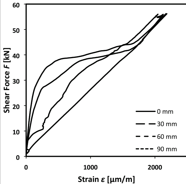
Figure C27.1: Shear-force-strain curves of shear resistance measurements of the anchorage of FRS-L-H CFRP strips externally bonded to concrete of class C12/15 along the bond length. Strain measurement at 0, 30, 60, 90 mm distances from the load application point.
