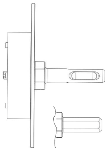
Countersunk setting 1)
