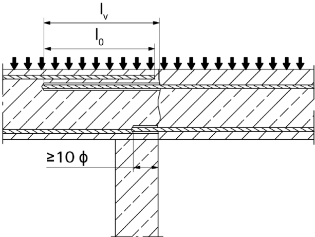
Figure A1.2: Overlap joint with existing reinforcement at a foundation of a column or wall where the rebar are stressed
