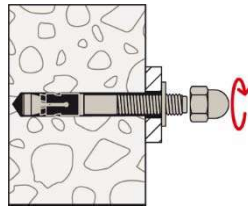
5.3: Turn on the fischer FAZ II Plus dome nut
