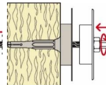
3. Put on setting tool
