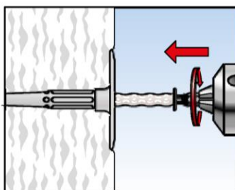
3. Set anchor by machine.
