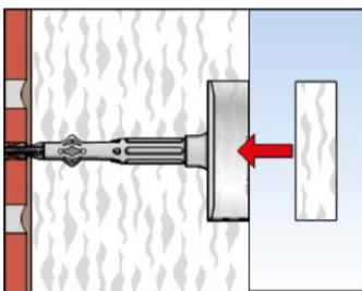
3. Put on polystyrene or mineral wool cap
