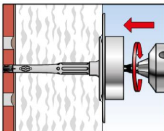
3. Set anchor by setting tool.
