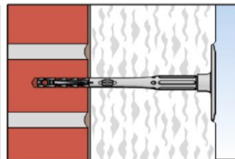
4. Correctly installed anchor
