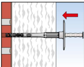
2. Insert anchor manually
