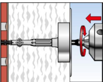
2. Insert anchor and set anchor by setting tool.
