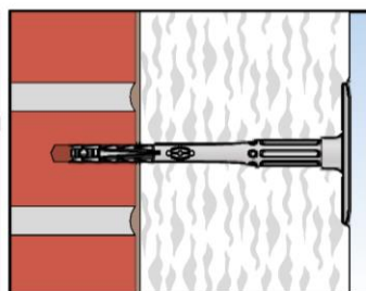
4. Correctly installed anchor
