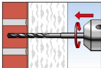
1. Drill hole by corresponding drilling method
