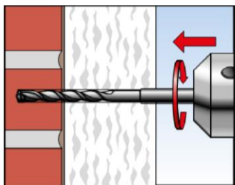
1. Drill hole by corresponding drilling method
