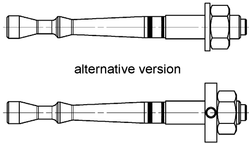
Highbond - Anchor FHB II Inject - A S
