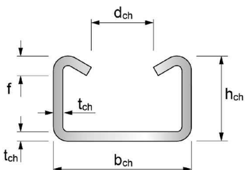
FES-C-40/25, -49/30, -54/33
