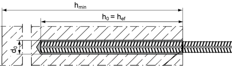
Reinforcing bar
