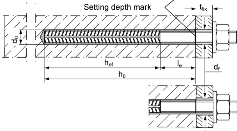
UPAT rebar anchor Pre-positioned anchor
