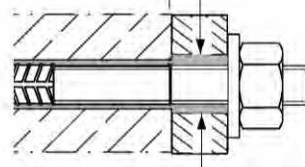
UPAT rebar anchor Push through anchor (annular gap filled with mortar)
