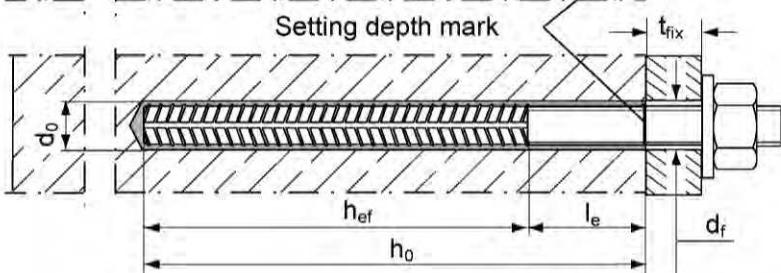
UPAT rebar anchor Pre-positioned anchor
