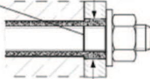
Upat threaded rod push through anchorage (annular gap filled with mortar)
