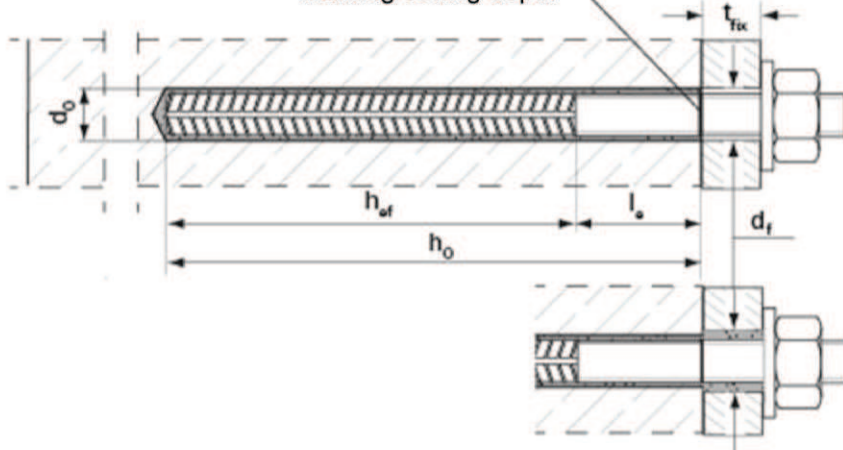
Upat rebar anchor push through anchorage (annular gap filled with mortar)
